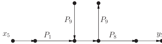
FIG. 10. The digraph T_5 .
