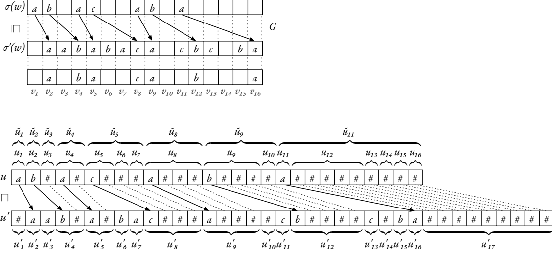
Figure 1: Exemplary reduction from \text{PEP}^{\text{reg}} to (\text{REG} \cap \square) \stackrel{?}{=} \emptyset , for the case \sigma(w) = abacaba , \sigma'(w) = aababacabcba .
